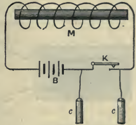
Fig 390.—Self-Induction of Current.
