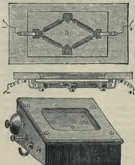
Fig. 428. — Crossley's Transmitter.
