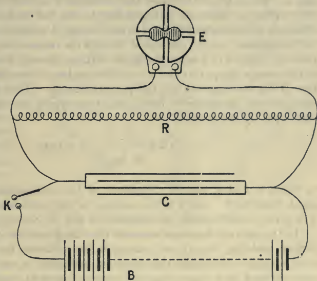
Fig. 744.—Measurement of High Resistance by Loss of Charge.
