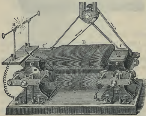
Fig. 444—Ladd's Machine.
