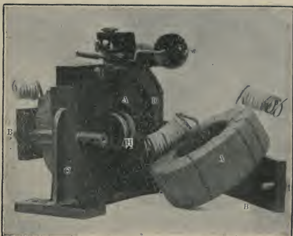
Fig. 788.—Details of E.C. Deflectional Wattmeters.
