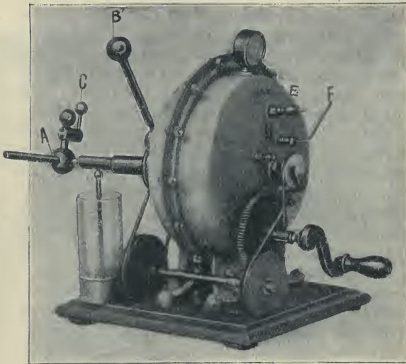
Fig. 93.—The Tudsbury Influence Machine.
