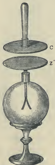
Fig. 136.—Volta's Condensing Electroscope.
