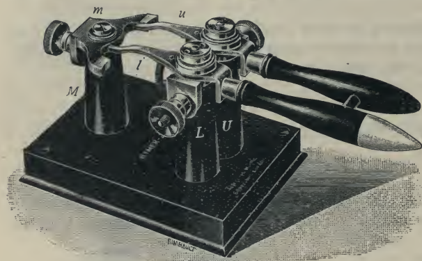
Fig. 750.—Rymer-Jones' High Insulation Key.
