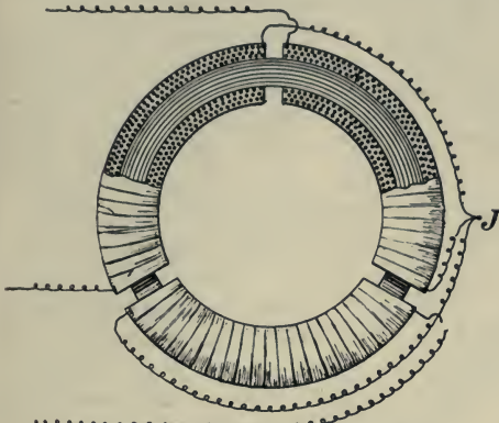
Fig. 582.—Tri-phase Rotating-Field Magnet, "Star" Connected.
