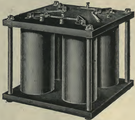
Fig. 549.—The "Nodon" Electric Valve.
