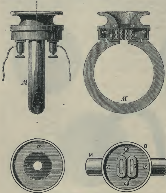
Fig. 425.—Ader's Telephone.
