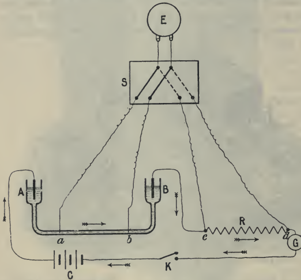
Fig. 743.—Measurement of Liquid Resistance by Fall of Potential.
