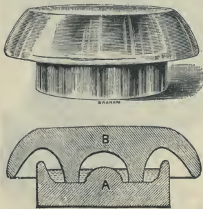
Fig. 190.—Glass and Oil Insulator.
