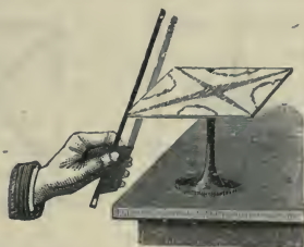
Fig. 416.—Production of Acoustic Sand Figures.
