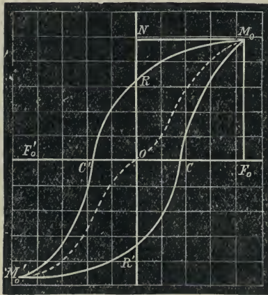
Fig. 254.—Typical Hysteresis Loop.
