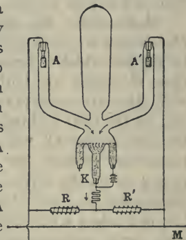
Fig. 666.—A.C. Mercury Lamp directly connected to Mains.
