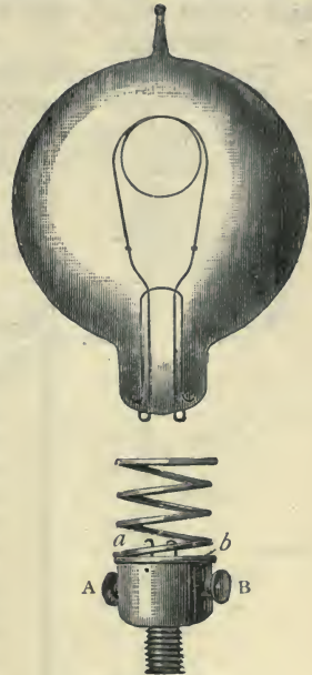
Fig. 200.—Swan's Early Lamp.
