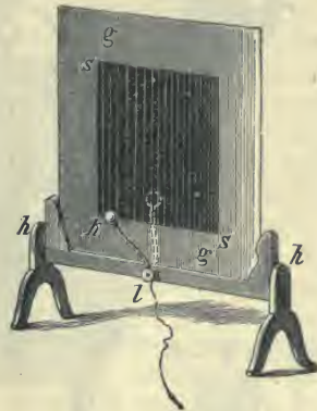
Fig. 103.—Franklin's Pane.
