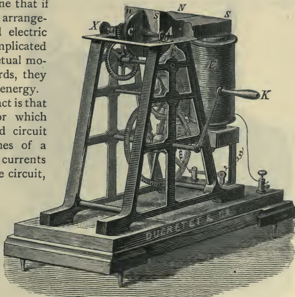
Fig. 491.—Mechanical Energy absorbed by Induced Currents.
