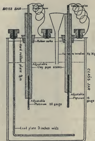
Fig. 635.—Price's Modification of Wehnelt's Interrupter.
