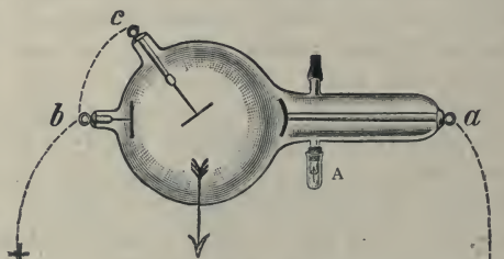
Fig. 687.—Tube with separate Anti-Kathode and Anode.
