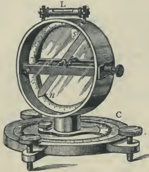
Fig. 35.—Simple Form of Dip Circle.
