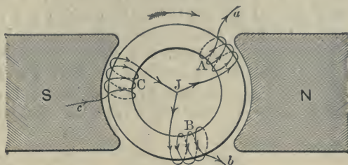
Fig. 524.—“Star” Connections of Three-phase Alternator.
