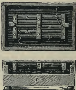
Fig. 429. — Ader's Transmitter.
