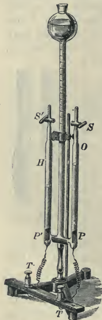
Fig. 175.—Hoffmann's Voltmeter.
