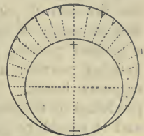
Fig. 486.—Difference of Potentials on a Commutator of a Gramme Machine.
