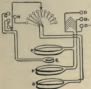
Fig. 777.—Circuits.
