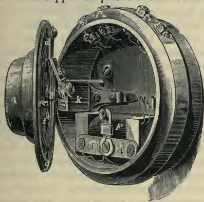
Fig. 431.—Berliner's Microphone.
