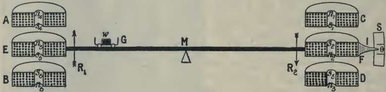
Fig. 733.—Principle of Lord Kelvin's Current Balances.
