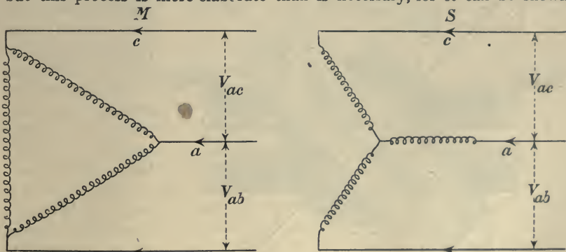
Fig. 791.—Measurement of Power in Three-phase Circuits.
