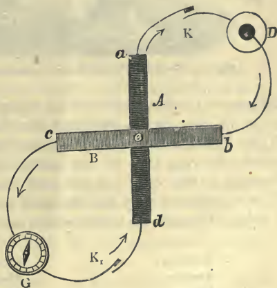
Fig. 158.—Peltier's Cross.
