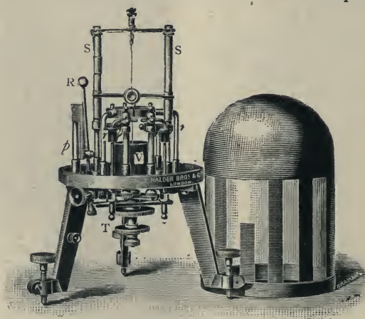
Fig. 349.—Ayrton, Perry & Sumpner's Quadrant Electrometer.
