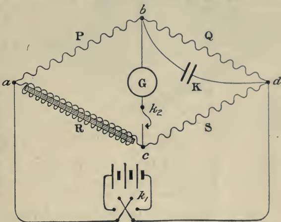
Fig. 770.—Maxwell's Method of Measuring Inductance.
