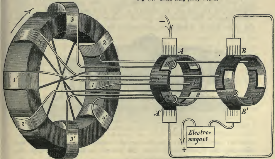
Fig. 472.—Connections of Brush Arc Light Machine.
