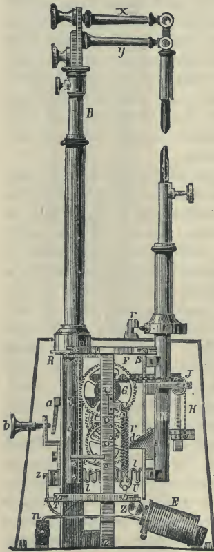
Fig. 217. —Serrin's Lamp.
