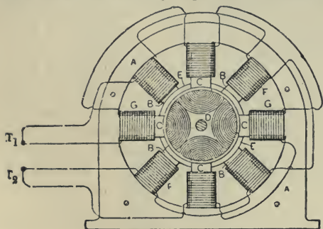
Fig. 605.—Tesla's Split-phase Motor.
