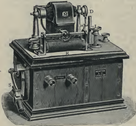
Fig. 625.—Motor-Driven Interrupter.
