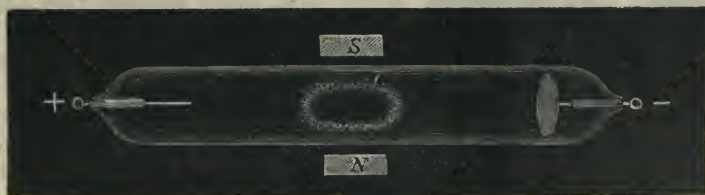
Fig. 674.—Action of a Magnet on a Discharge in a High Vacuum.
