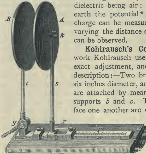
Fig. 99.—Reiss' Condenser.
