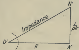
Fig. 522.—Construction for Impedance.
