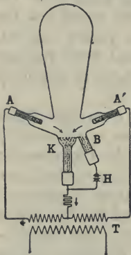
Fig. 665.—Connections for A.C. Mercury Lamp.
