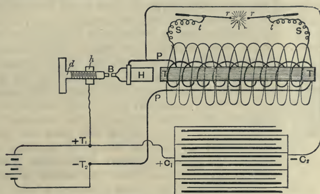
Fig. 395.—Connections of a Battery Induction Coil.
