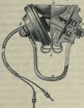
Fig. 426.—Gray's Telephone.
