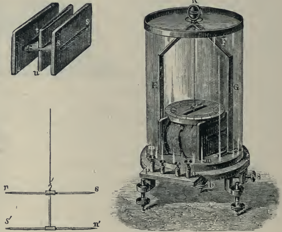
Fig. 311.—The Astatic Galvanometer.
