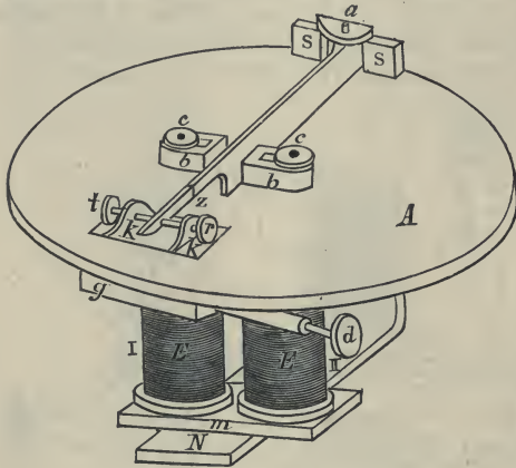
Fig. 371.—Siemens' Polarised Relay.
