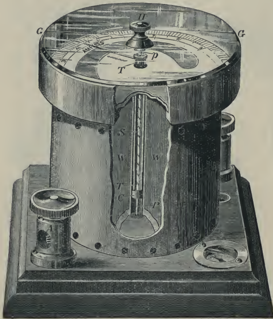
Fig. 316.—Ayerton and Perry's "Magnifying Spring" Ammeter.
