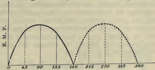
Fig 456.—Commuted Alternate Currents.
