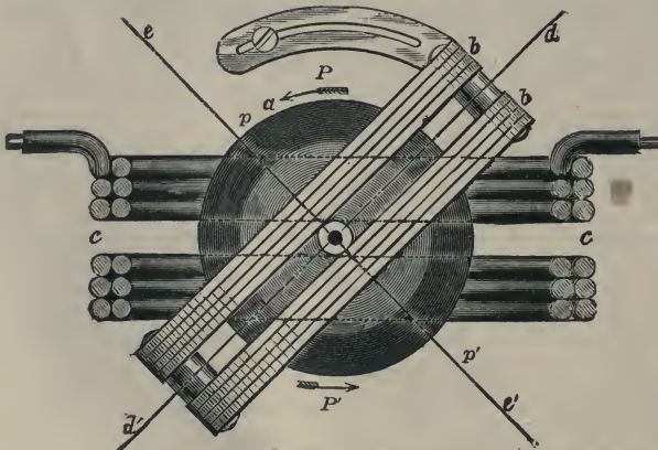
Fig. 793.—Electrical Circuits of Shallenberger's Meter.
