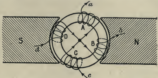
Fig. 527.—Star Connection of Two- (or Four-) phase Alternators.
