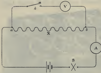
Fig. 748.—Ammeter and Voltmeter Method of Measuring Low Resistances.
