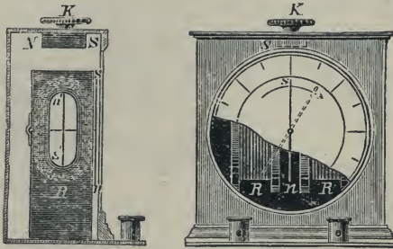
Fig. 310.—The Vertical Galvanoscope.
