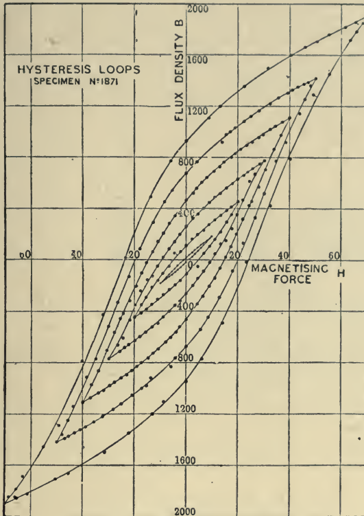
Fig. 275.—Hysteresis Loops of Copper Alloy.
