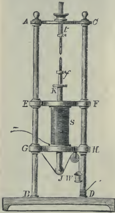
Fig. 215.—Archereau's Regulator.
