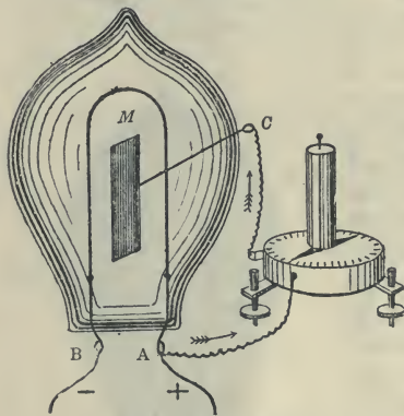
Fig. 209.—Connections for Showing the Edison Effect.
