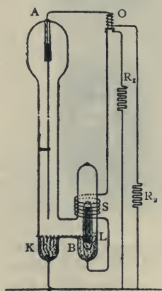
Fig. 664.—Plunger Method of starting a Mercury Arc.
