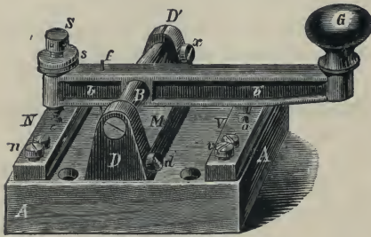
Fig. 372.—The Morse Key.
