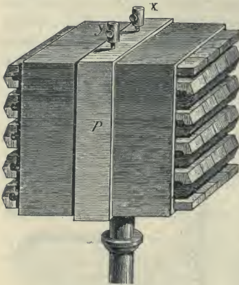
Fig. 162.—The Thermopile.
