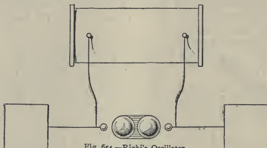
Fig. 654.—Righi's Oscillator.
