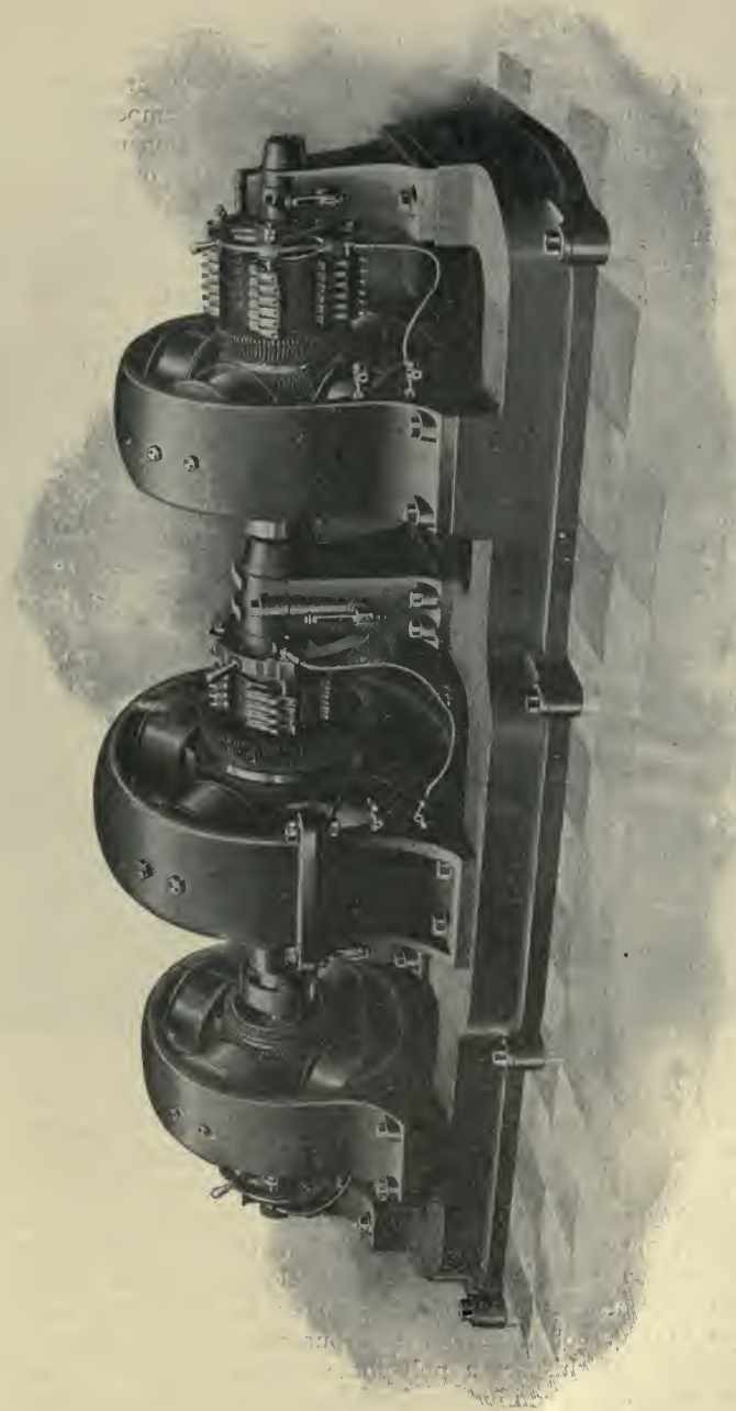
Fig. 607.—Continuous Current Transformer (C-coupled Plant)
