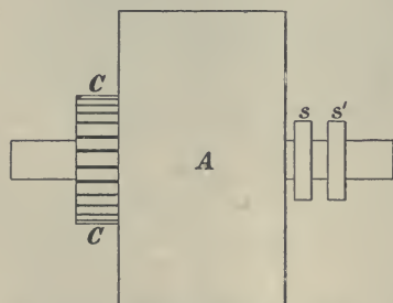
Fig. 614.—Armature with Commutator and Slip Rings.
