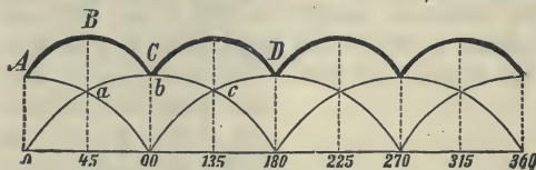
Fig. 462—E. M. F.'s of Two Pairs of Coils in Series.
