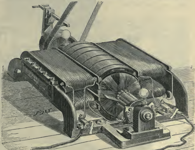
Fig. 493.—Early Siemens' Machine.
