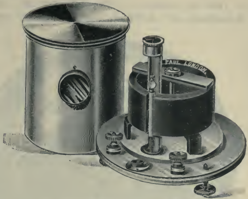
Fig. 716.—Ayrton-Mather Moving-coil Galvanometer.
