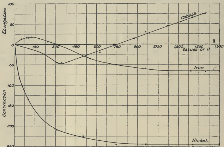
Fig. 269—Changes of Length on Magnetisation.
