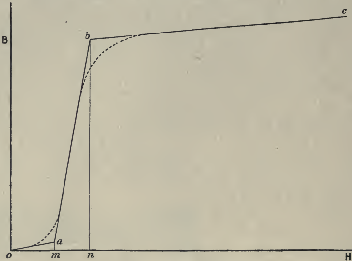
Fig. 283.—Stages of Magnetisation.
