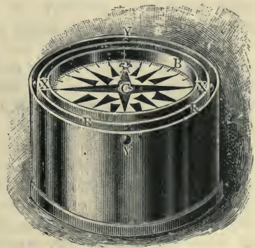
Fig. 10.—Mariner's Compass.
