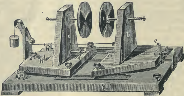
Fig. 100.—Kohlrausch's Condenser.
