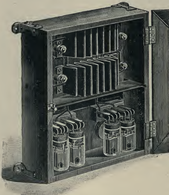
Fig. 354.—Edison's Public Supply Meter.
