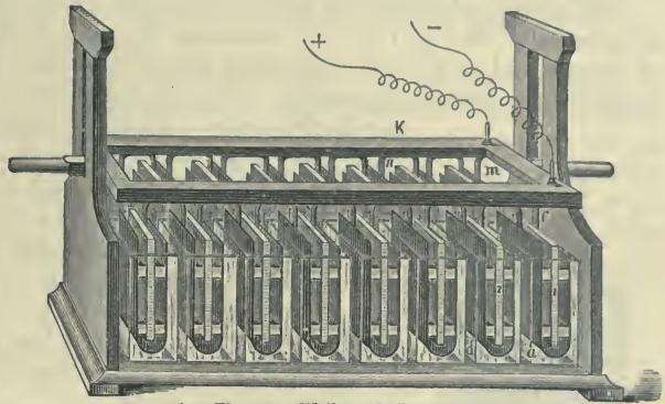
Fig. 133.—Wollaston's Battery.
