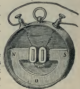
Fig. 306.—Polarised Electro-magnet of Gower Telephone.
