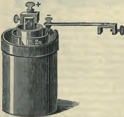
Fig. 145.—A Bunsen Cell.
