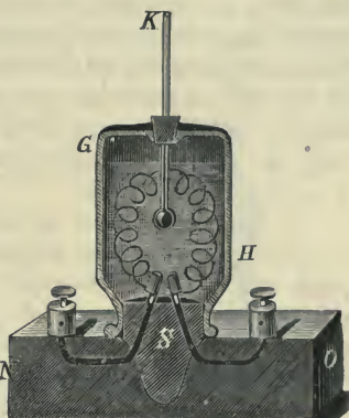
Fig. 195.—Lenz's Current Calorimeter.
