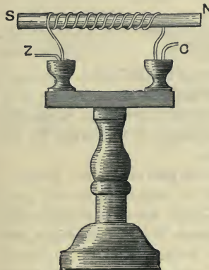
Fig. 249.—Sturgeon's Straight Electro-magnet.
