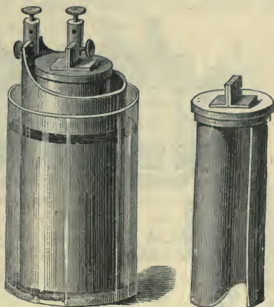
Fig. 141.—A Grove's Cell. Fig. 142.—The Platinum.
