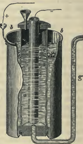
Fig. 155.—Daniell's Cell.
