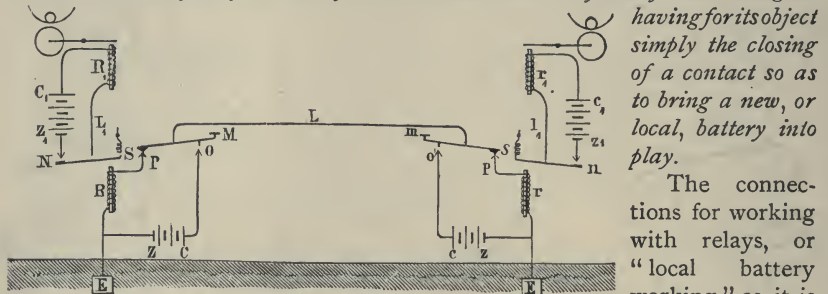
Fig. 369.—Relay Connections.
