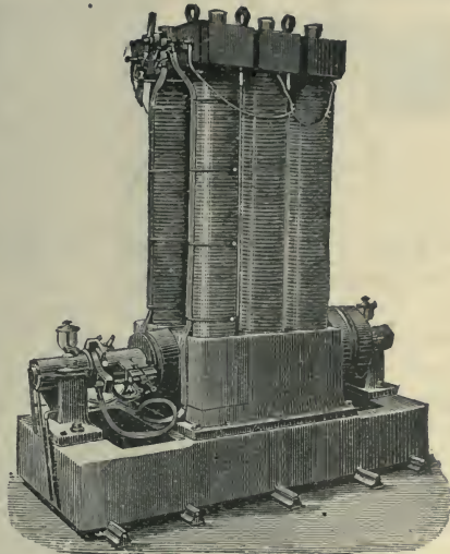
Fig. 497.—Early Edison Machine.
