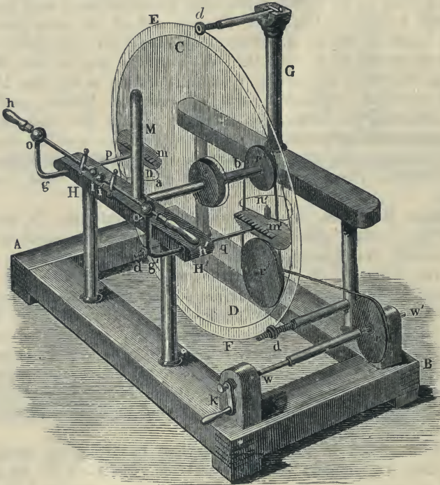
Fig. 83.—Holtz Machine.
