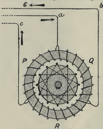
Fig. 594.—Drum-Wound Rotor.
