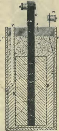
Fig. 153.—Section of Lessing's Cell.
