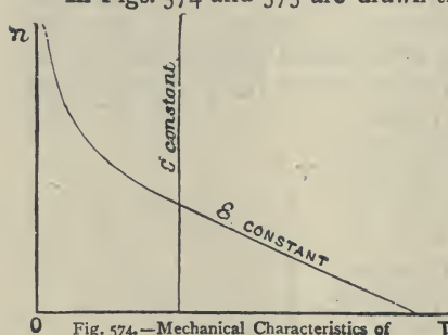
Fig. 574.—Mechanical Characteristics of a Series Motor.
