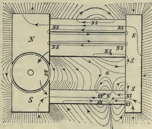
Fig. 476.—Magnetic Leakage in early form of Dynamo.
