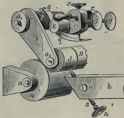
Fig. 378.—Details of the Morse Embosser.
