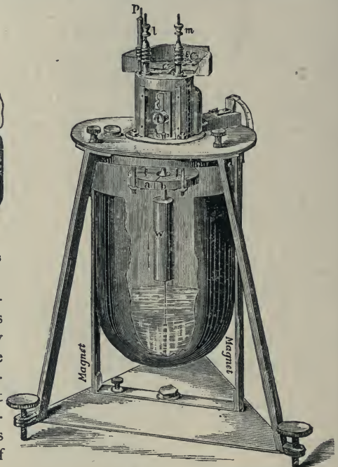
Fig. 347.—Lord Kelvin's Quadrant Electrometer.
