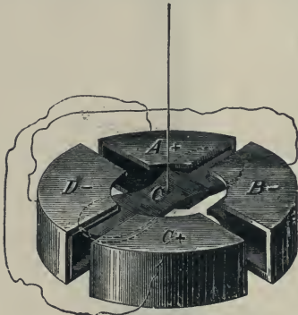
Fig. 346.—The Quadrants in Lord Kelvin's Electrometer.
