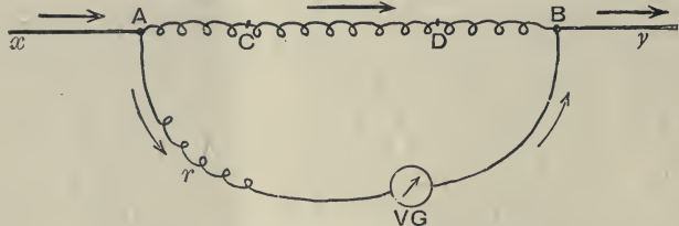
Fig. 342.—Measurement of Potential Differences
