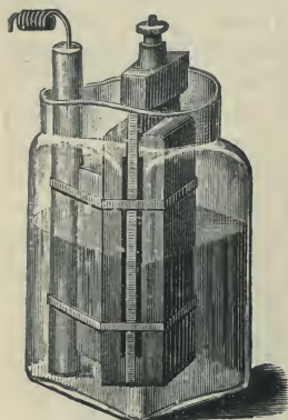
Fig. 149.—Agglomerate Leclanché's Cell.
