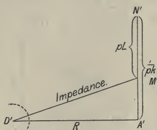
Fig. 523.—Permittance and Inductance combined.
