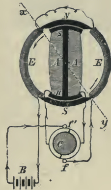
Fig. 571.—Section.
