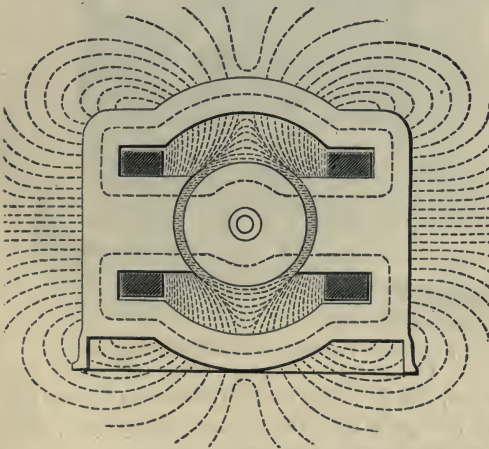
Fig. 507.—Leakage Field of Iron-clad Dynamo.
