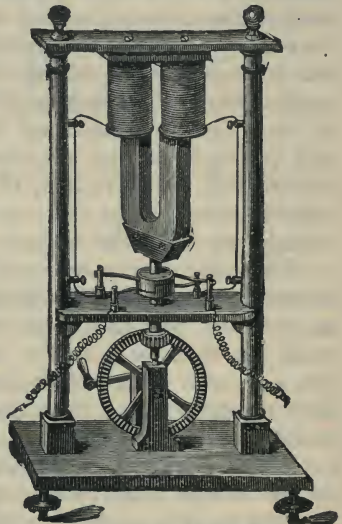
Fig. 438.—Pixii's Machine.
