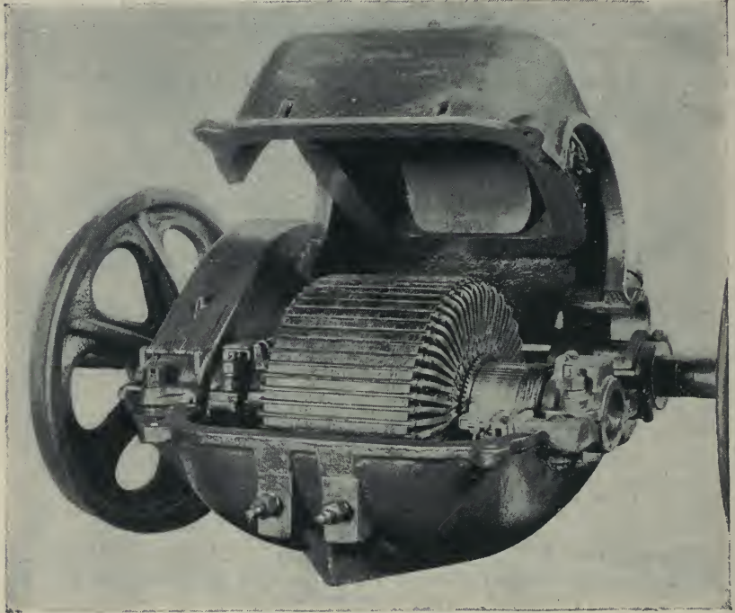
Fig. 569.—Fifty Horse-power Waterproof Railway Motor (1892).
