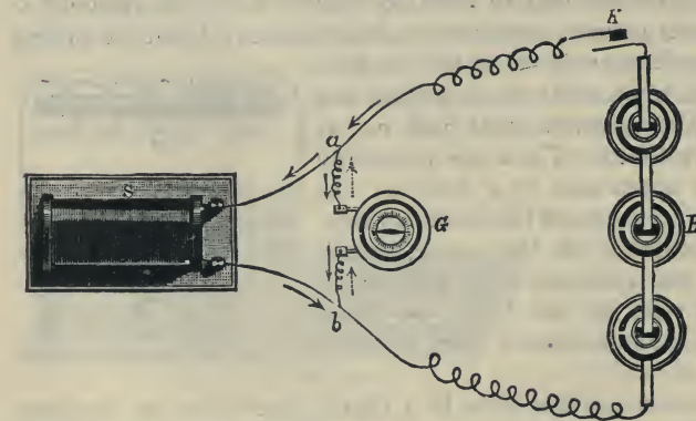
Fig. 391. —Experiment on Self-Induction.
