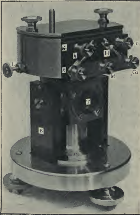
Fig. 763.—The Duddell Permanent Magnet Oscilligraph.
