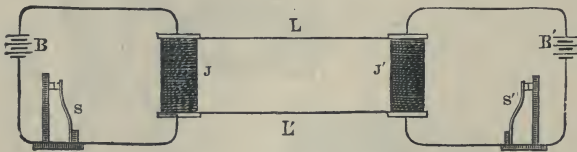
Fig. 411.—Berliner's Transmitter.
