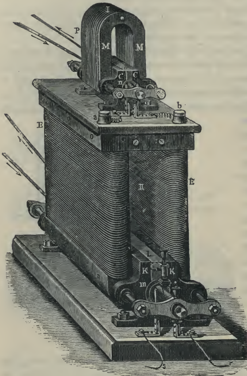
Fig. 442.—Wilde's Machine.
