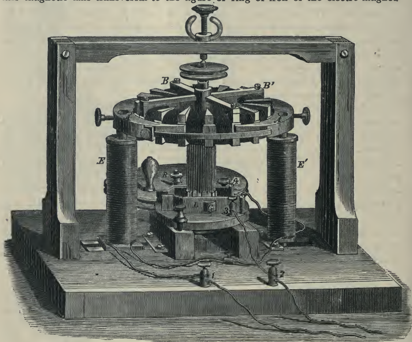
Fig. 561.—Pacinotti's Machine.
