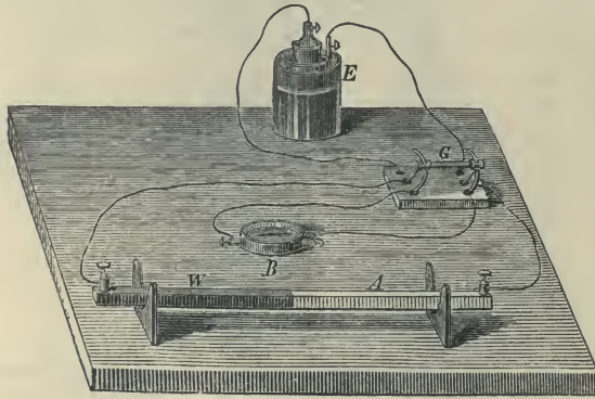
Fig. 160.—Peltier's Bar.
