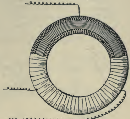
Fig. 583.—Tri-phase Rotating-Field Magnet, "Mesh" Connected.
