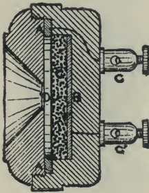
Fig. 435.—Hunning's Transmitter.
