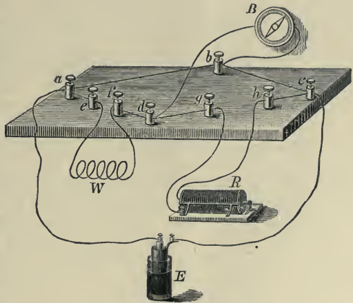
Fig. 333.—Wheatstone's Bridge.
