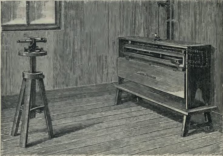
Fig. 357.—Gauss and Weber's Telegraph.
