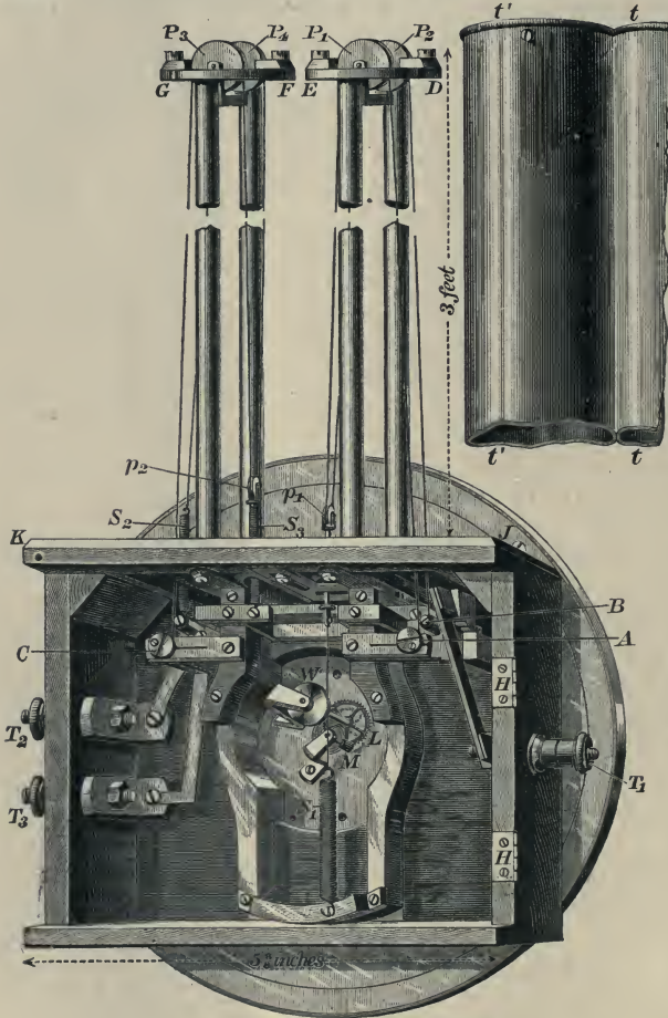
Fig. 344.—Cardew's "Hot-wire" Voltmeter.
