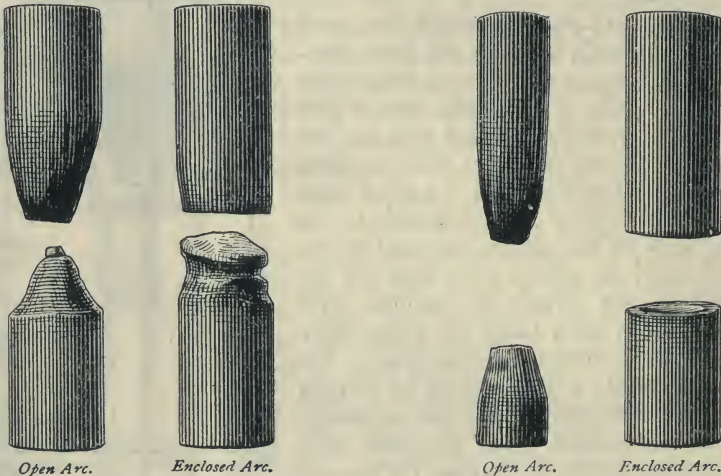
Fig. 231.—Arcs at 6 Amperes and 45 Volts.
