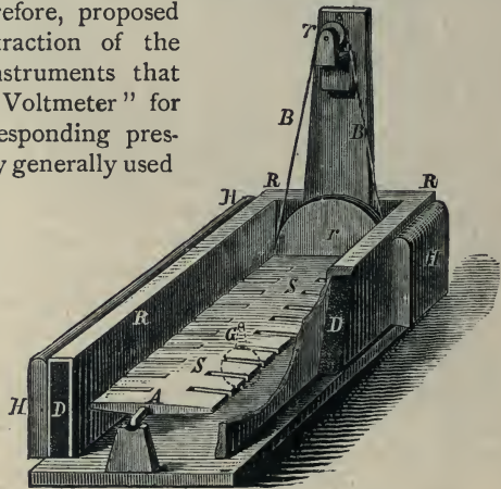
Fig. 313.—Deprez's Galvanometer.
