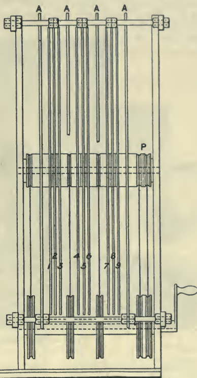
Fig. 89.—Pidgeon's Influence Machine (side).
