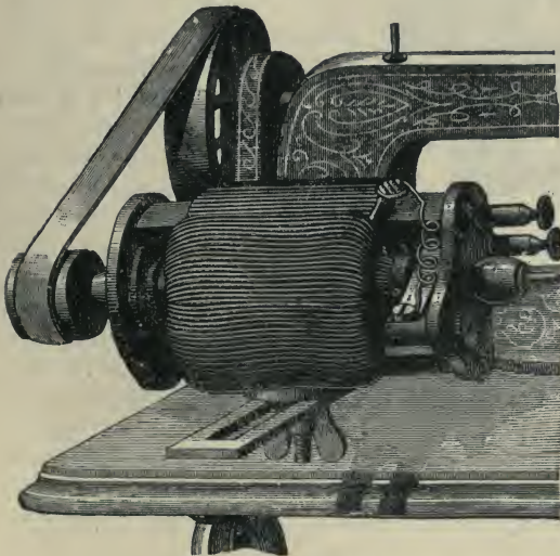
Fig. 570.—Griscom's Motor.
