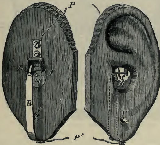
Fig. 406.—Reis's Telephone.
