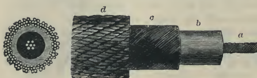
Fig. 365.—The First Atlantic Cable.
