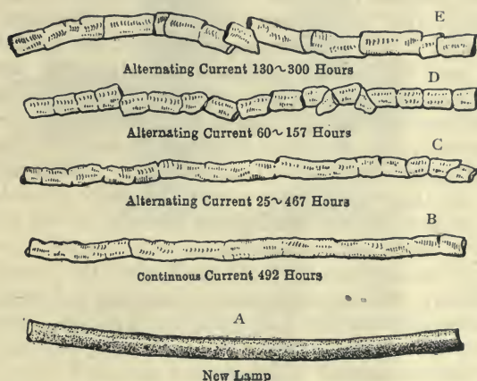
Fig. 211.—Effect of various kinds of current on a Tantalum Filament.
