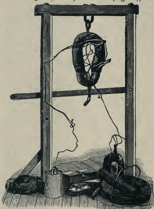
Fig. 292.—Henry's Electro-magnet.
