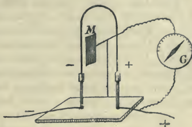
Fig. 210.—"The Edison Effect" in the Open Air.
