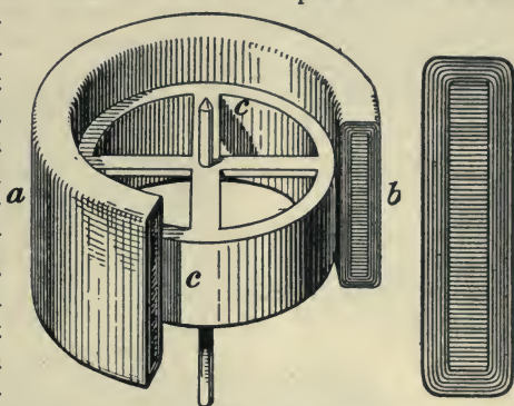
Fig. 589.—Copper Cylinder placed in a Rotating Magnetic Field.
