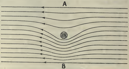
Fig. 447.—Lines of Force of a Straight Current placed in a Uniform Field.
