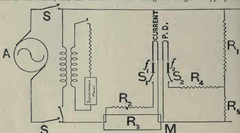
Fig. 764.—Connections of Oscillagraph for High-voltage Circuits.
