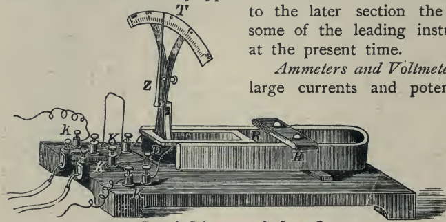
Fig. 312.—Deprez's Galvanometer for Large Currents.
