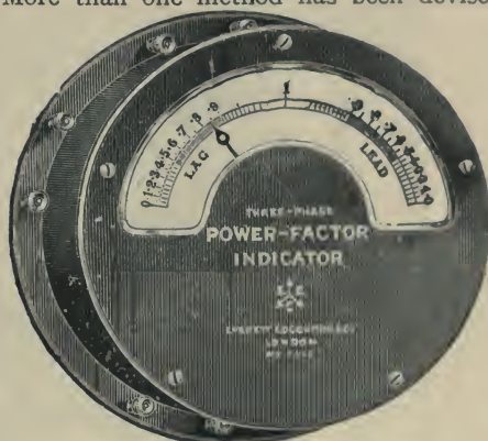
Fig. 793.—E.E.C. Power-factor Indicator.
