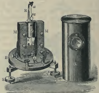
Fig. 715.—D'Arsonval's (Maxwell) Galvanometer.
