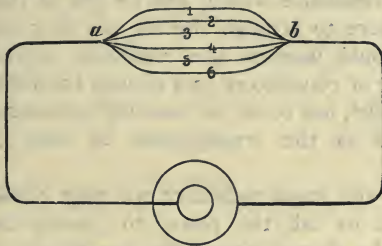
Fig. 171.—Divided Circuit.
