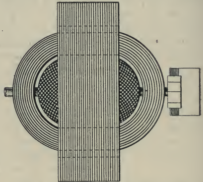
Fig. 604.—Plan of Mono-phase Induction Motor.
